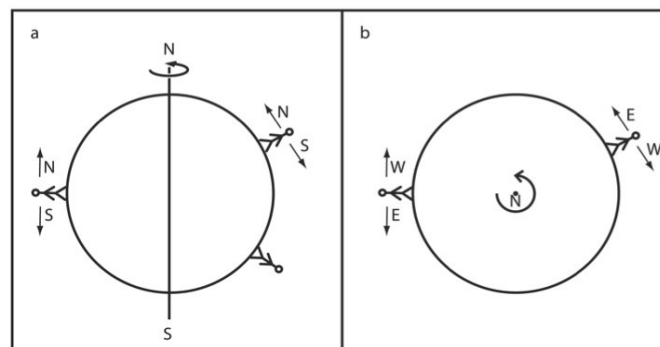
Figure 3: Determining directions for a person on globe (3a. Earth viewed from the plane of the equator; 3b. Earth viewed from the North Pole)
